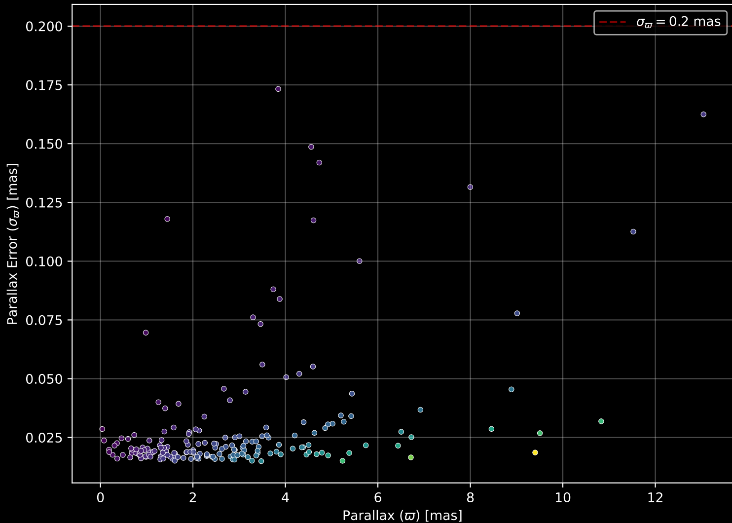
APOGEE DR17 Field: [224+49_btx] Parallax Quality (n= 185)
