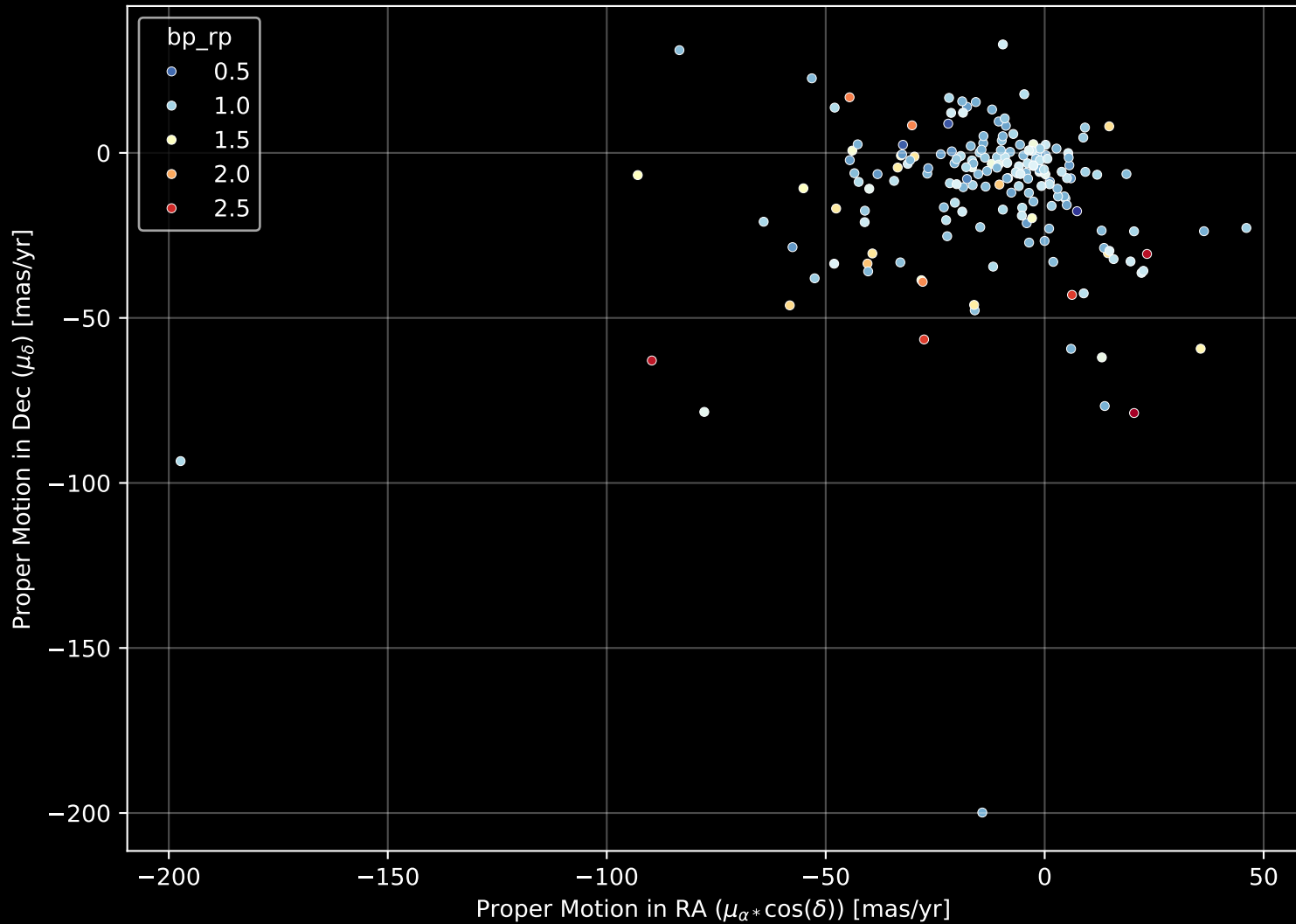
APOGEE DR17 Field: [224+49_btx] Proper Motion Diagram (n= 185)
