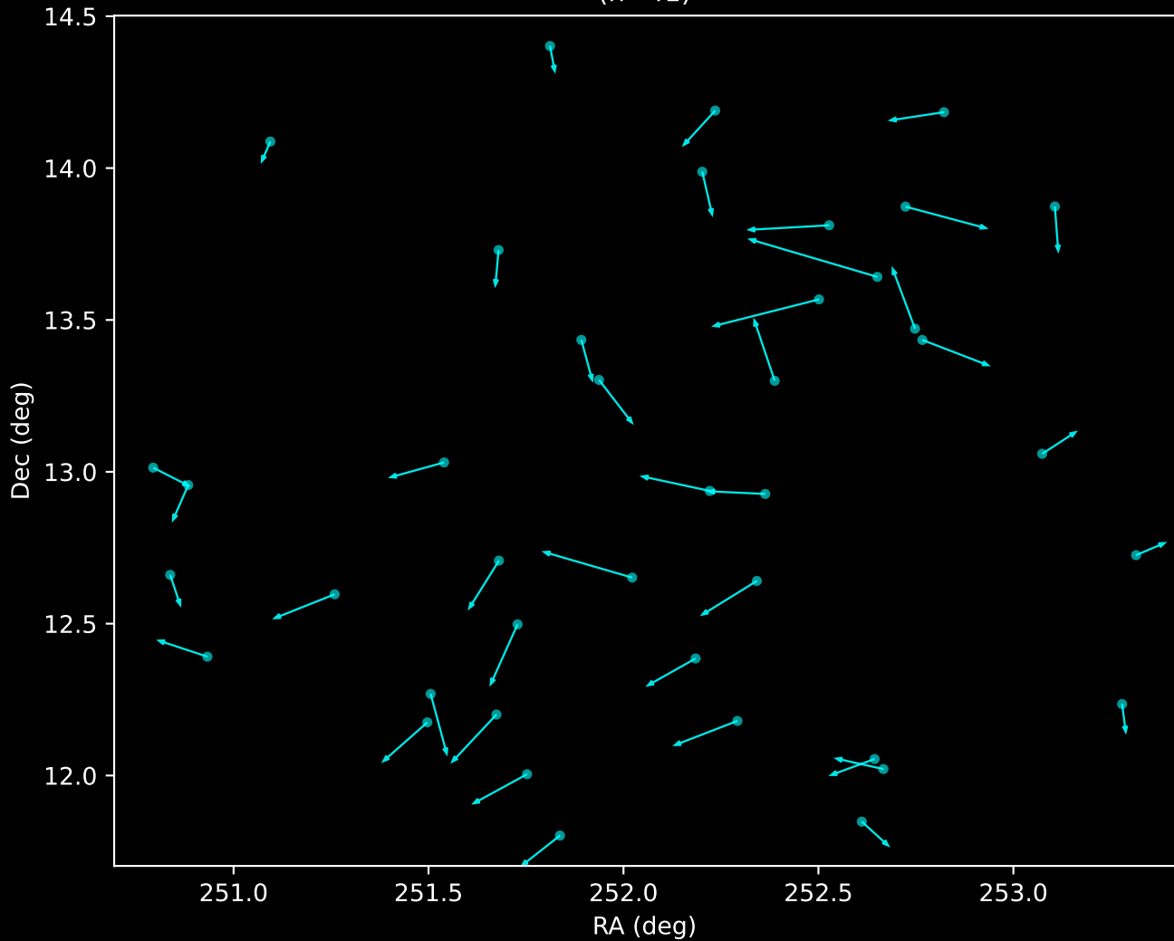
APOGEE DR17 Noise Stream Proper Motion Vectors (n=41)
