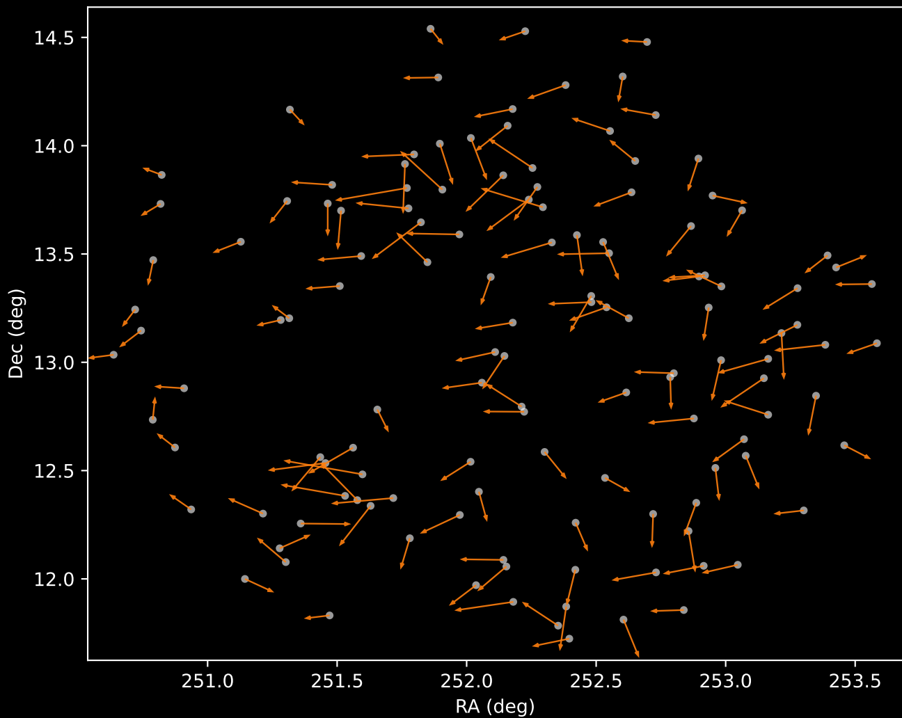
APOGEE DR17 Cluster 2 Proper Motion Vectors (n=130)
