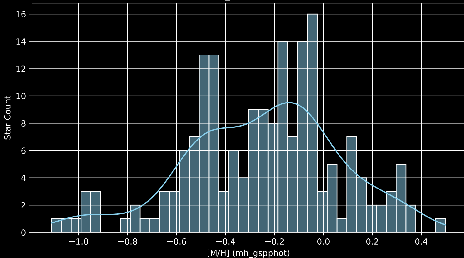
APOGEE DR17 Field: [224+49_btx [M/H] (mh_gspphot) (n= 184)
