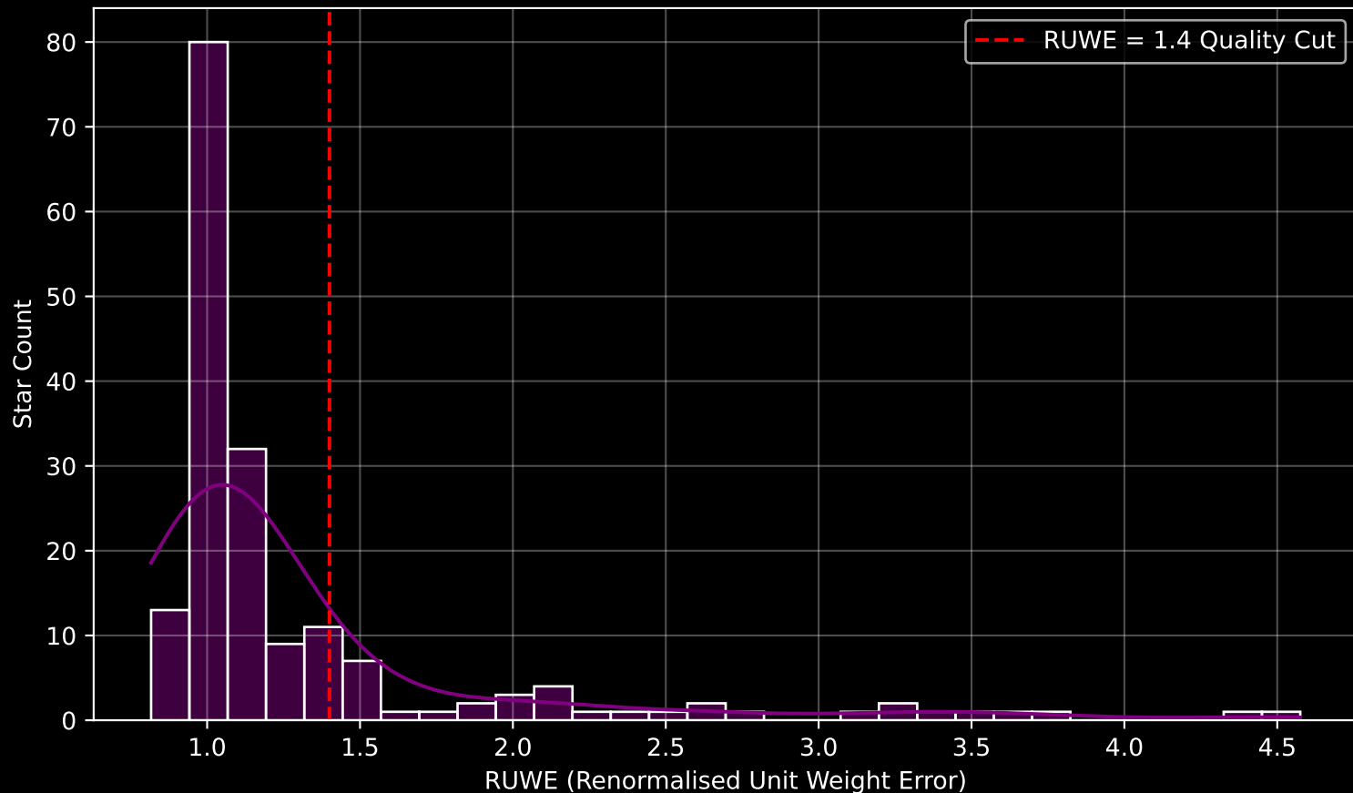
GAPOGEE DR17 Field [224+49_btx] RUWE Distribution (n= 178)
