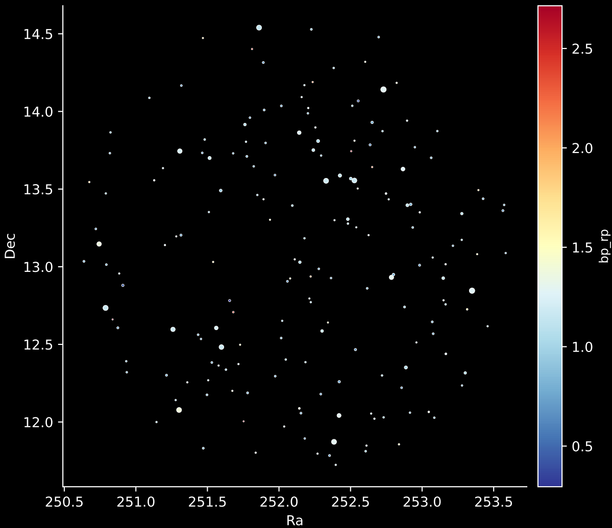
APOGEE DR17 Field: [224+49_btx] Stars: 185
