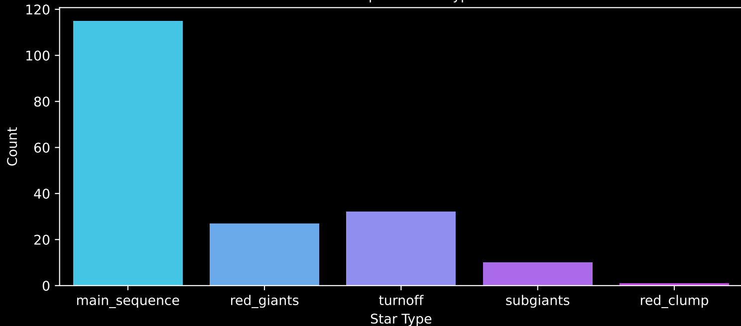
APOGEE DR17 Field: [224+49_btx] Count plot of Star Type
